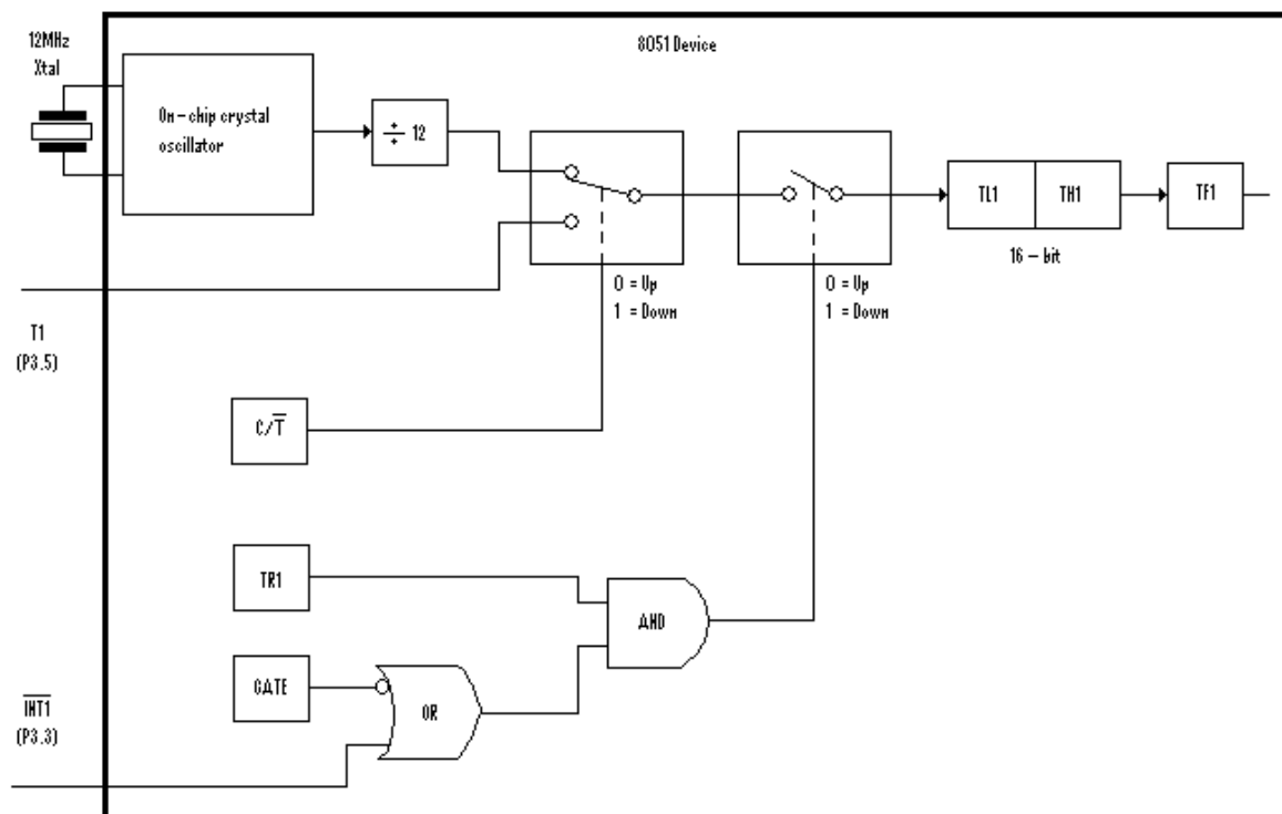
Figure 2-2 Timer 1 Mode 1
