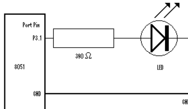
Figure 11-1 Port Driving LED (pin High = LED on)
