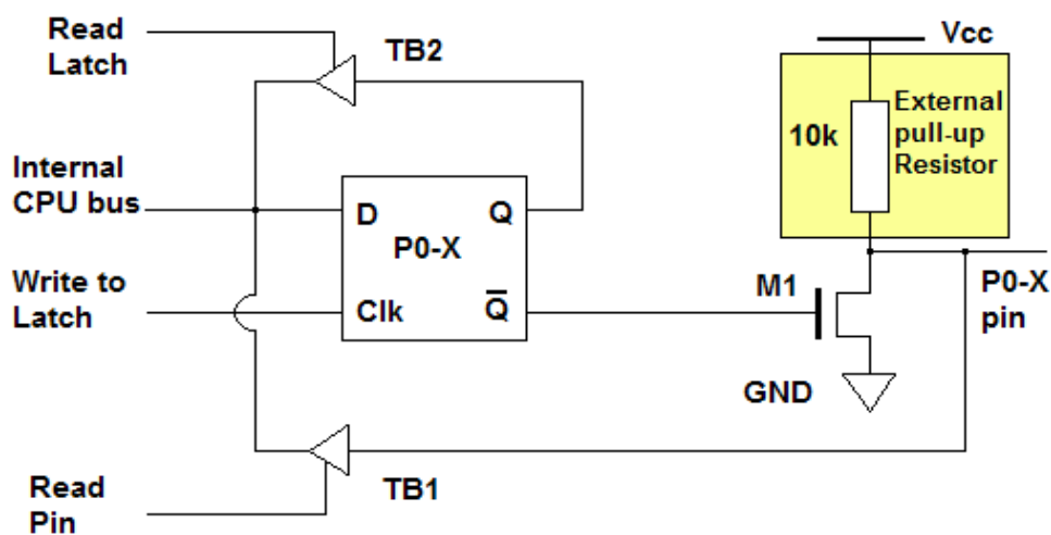
Figure 1-2 Pull-Up resistors
