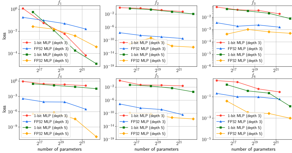
Figure 1: Verification experiment for scaling law for 1-bit neural networks. Minimum training loss of scaling number of parameters for MLP model to learn complicated functions f_1, f_2, f_3, f_4, f_5 and f_6 , and these function is defined in Section 6.1.
