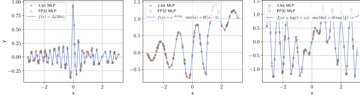
Figure 2: This plot shows the difference between the predicted and actual values of the functions on the test dataset. We tested three complex functions, as seen in the images, and the performance of the 1-bit model is nearly identical to that of the standard 32-bit floating-point model.
