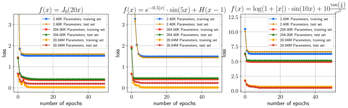
Figure 3: This plot shows the \ell_2 difference between both the training and test points and the predicted points throughout the training phase for different model sizes and parameter counts. Each plot demonstrates how the error decreases as training progresses, highlighting the impact of model size on both training and test performance.
