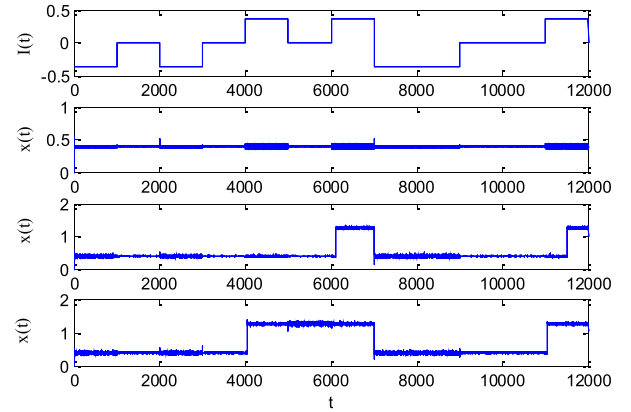
Fig. 6. Panels from top to bottom, the input signal, the responses of the system to periodic forcing, Gaussian noise, and periodic forcing together with Gaussian noise. Here, A = 0.05 , D = 0.03 , and f = 0.01 .
