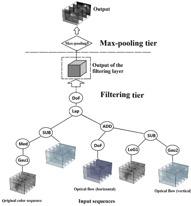
Fig. 5. Illustration of a possible learned-structure. All the 3D operators and pooling functions used in the structure are randomly selected through the GP evolution.
