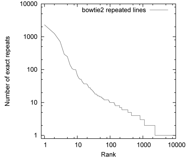
Fig. 5. Distribution of repeated Bowtie2 C++ code, after macro expansion, follows approximately Zipf's law, which predicts a straight line with slope of -1.
