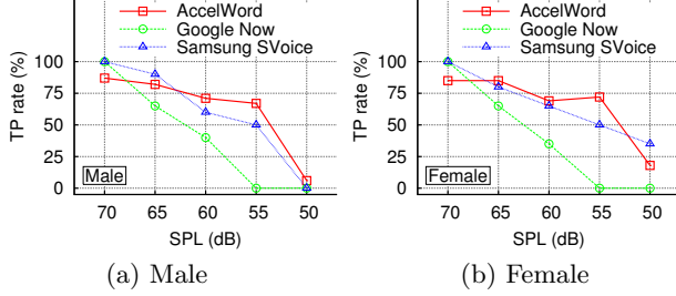
Figure 18: Accuracy Comparison with Google Now and Samsung S Voice
