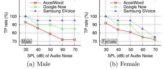
Figure 19: True Positive Rate vs. Audio Noise SPL
