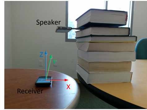
Figure 6: Experiment Setup
