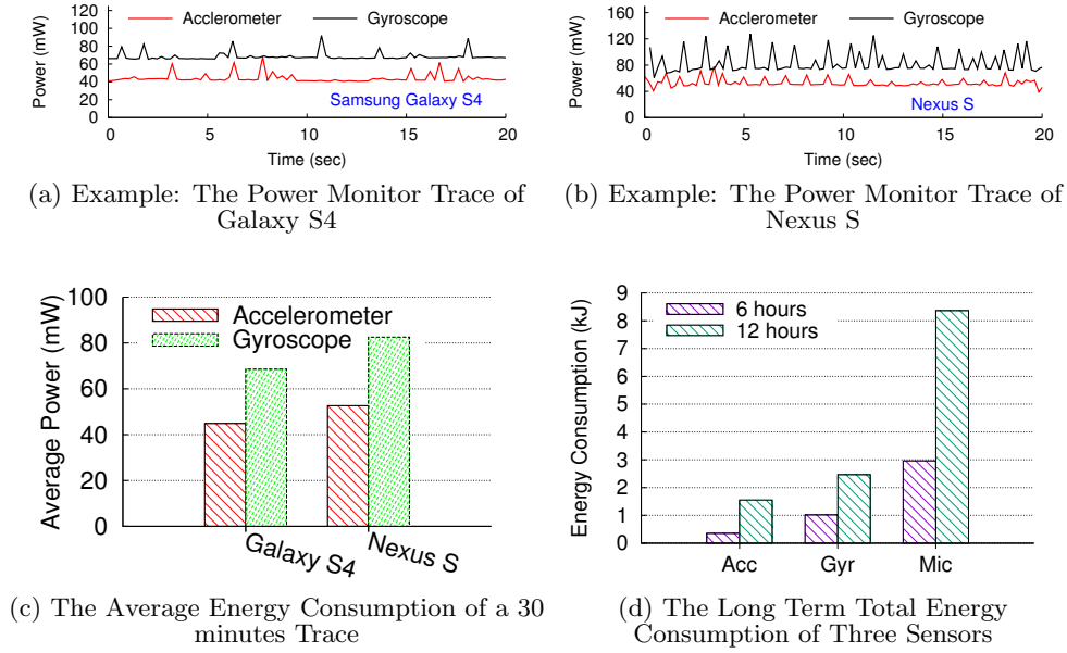
Figure 8: The Energy Consumption of Accelerometer, Gyroscope and Microphone
